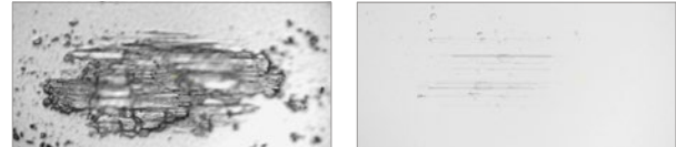
COF*: 0,76 Pure silver without Sealing
